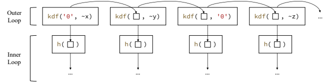
Figure 13: Nested loop example.
